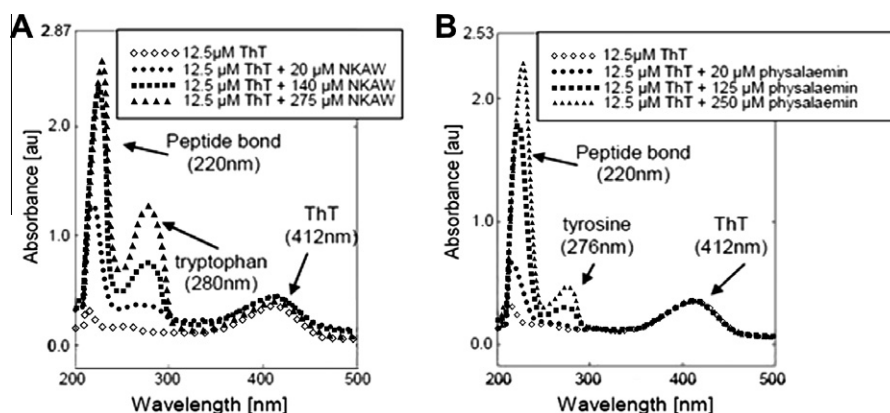
Fig. 4. Absorption spectra of 12.5 \mu M ThT in the presence of increasing concentrations of NKA (A) and physalaemin (B). The absorbance of ThT is unchanged, suggesting no interaction with the tachykinins.
