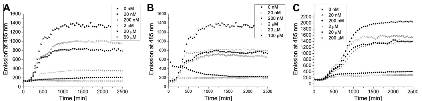
Fig. 2. ThT fluorescence as a function of time of A \beta (1–40) alone or in the presence of different concentrations of SPW (A); NKBW (B); or NKA (C); t = 0 indicates the time of A \beta (1–40) dissolution in the working buffer (see text). The neuropeptide concentrations are indicated next to each curve.
